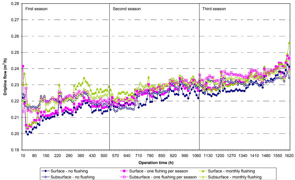
Fig. 2. Average emitter 1 lateral flow rate for every 10 h of experiment.
