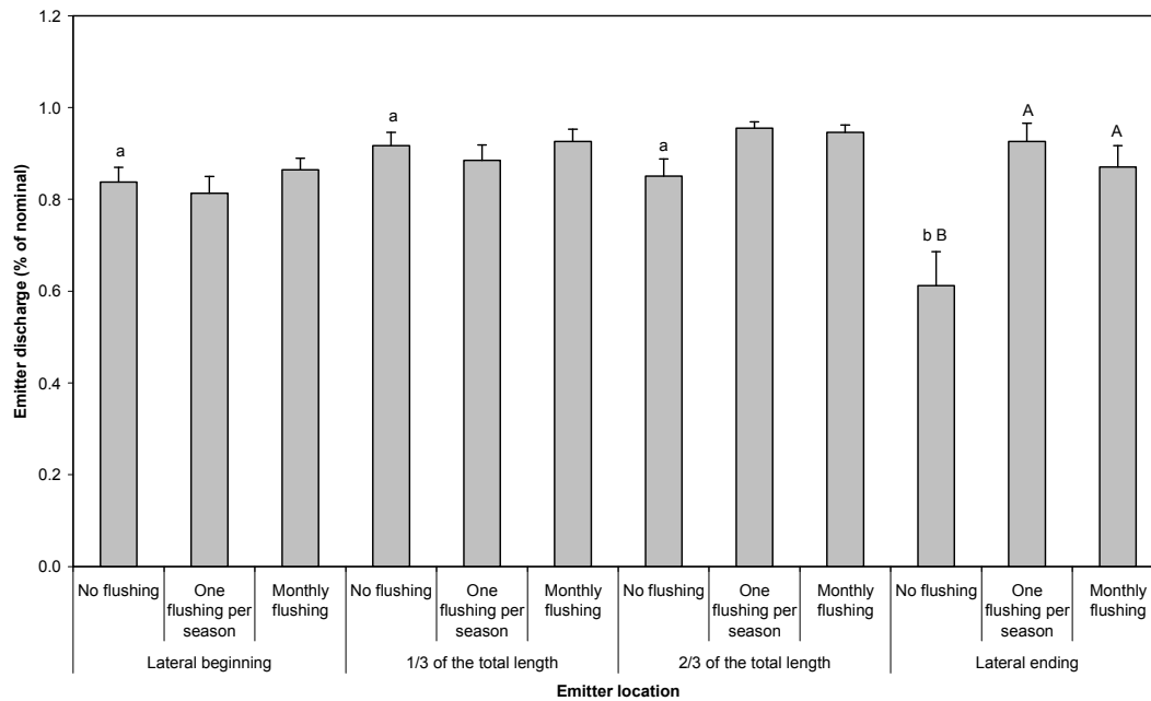
Fig. 5. Average relative emitter discharge and standard error after 1620 h for the three flushing frequency treatments for the different locations. For each flushing frequency treatment, different lowercase letters mean significant differences ( P < 0.05 ) among sampling locations. For each emitter location, different uppercase letters mean significant differences ( P < 0.05 ) among treatments.
