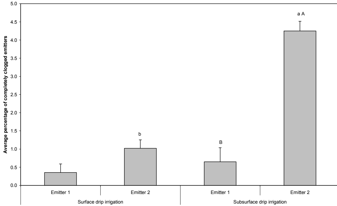
Fig. 6. Average percentage of totally clogged emitters and standard error at the end of the experiment. For each emitter, different lowercase letters mean significant differences ( P < 0.05 ) among irrigation system. For each irrigation system, different uppercase letters mean significant differences ( P < 0.05 ) among emitters.
