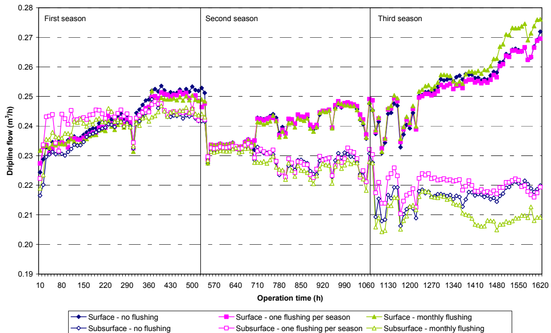
Fig. 3. Average emitter 2 lateral flow rate for every 10 h of experiment. Dotted lines show a period where the system was operating but the data was missed as the instrumentation was not working properly.
