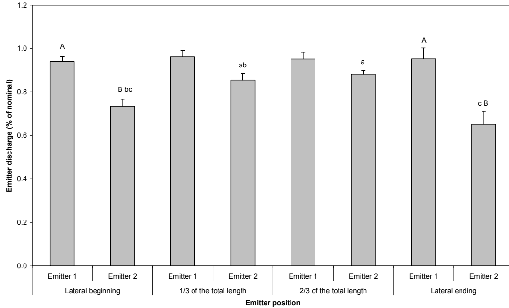
Fig. 4. Average relative emitter discharge and standard error after 1620 h for Emitter 1 (pressure compensating) and Emitter 2 (nonpressure compensating) for the different locations. For each emitter, different lowercase letters mean significant differences ( P < 0.05 ) among sampling locations. For each emitter location, different uppercase letters mean significant differences ( P < 0.05 ) among emitters.
