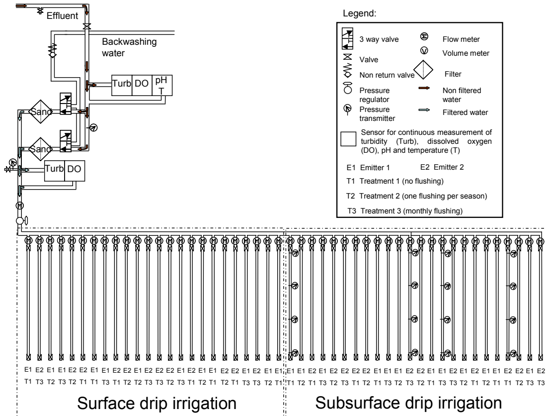
Fig. 1. Hydraulic diagram of the microirrigation system and location of monitoring and control equipment.
