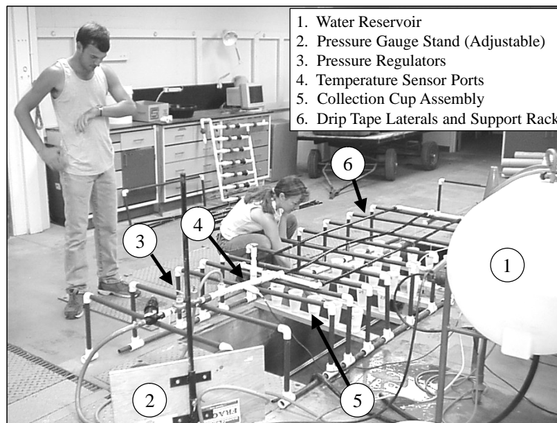
Figure 1. Lab setup to measure drip tape emitter discharge rates.
