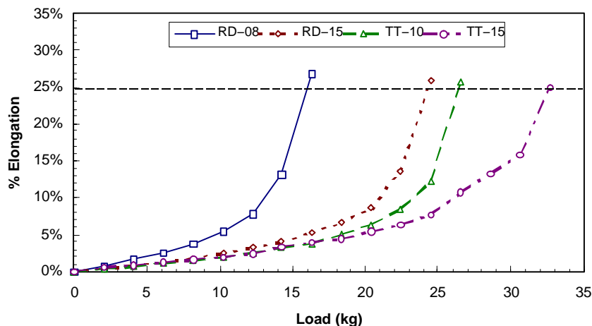
Figure 2. Resistance to tensile stress expressed as percent elongation of 152-cm long sample of product in response to loading. Loading was ceased at 25% elongation. Average results for each of the four tested products are shown.
