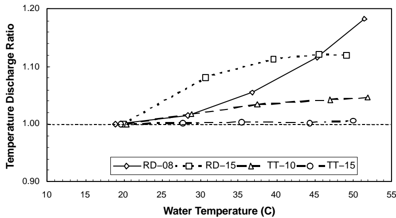
Figure 5. Temperature discharge ratio (TDR) values as affected by water temperature for the RD-08 , RD-15 , TT-10, and TT-15 products when operated at a pressure of 55 kPa.
