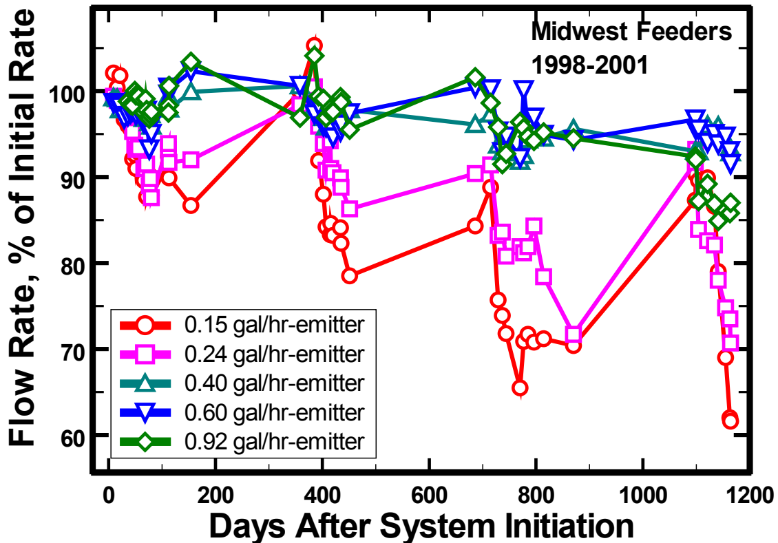
Figure 1. Measured flow rates for five dripline types with different emitter flow rates using lagoon wastewater, Midwest Feeders, KS, 1998-2001.
