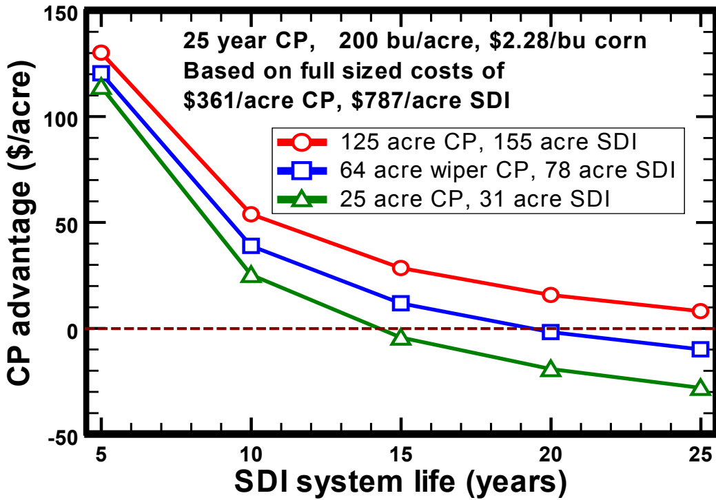
Figure 3. CP economic advantage as affected by field size, shape, and SDI system life.
