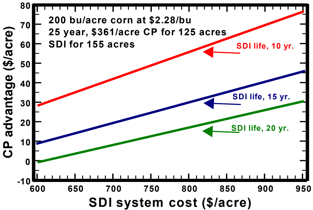
Figure 4. CP economic advantage as affected by SDI system life and cost.
