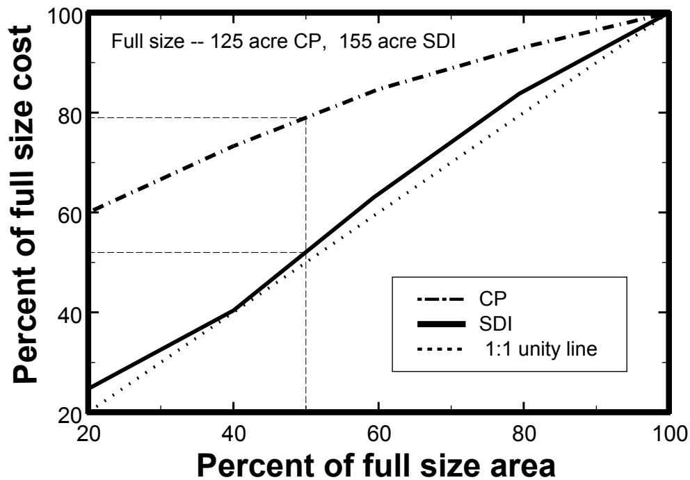
Figure 1. CP and SDI system costs as related to field size. (O'Brien et al., 1997)
