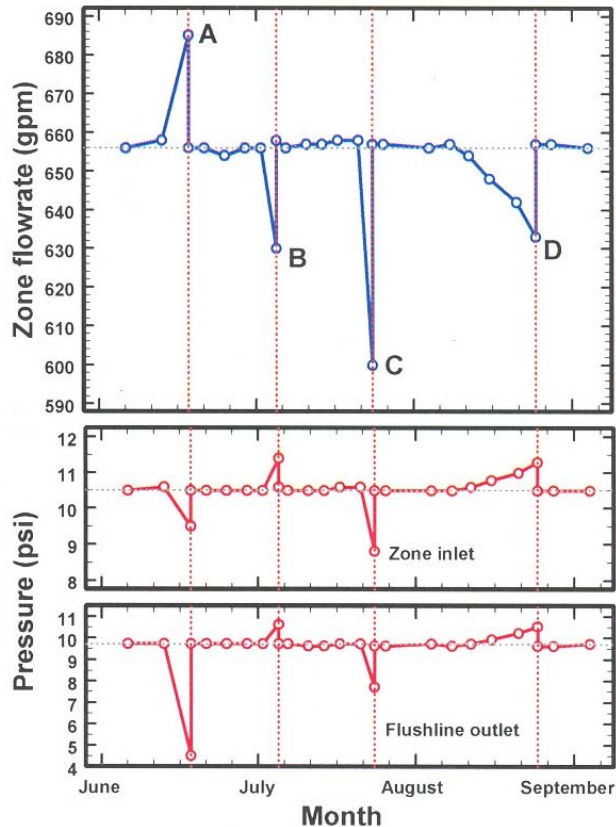
Figure 3. Hypothetical example of how pressure and flowrate measurement records could be used to discover and remediate operational problems (Lamm and Camp, 2007).
