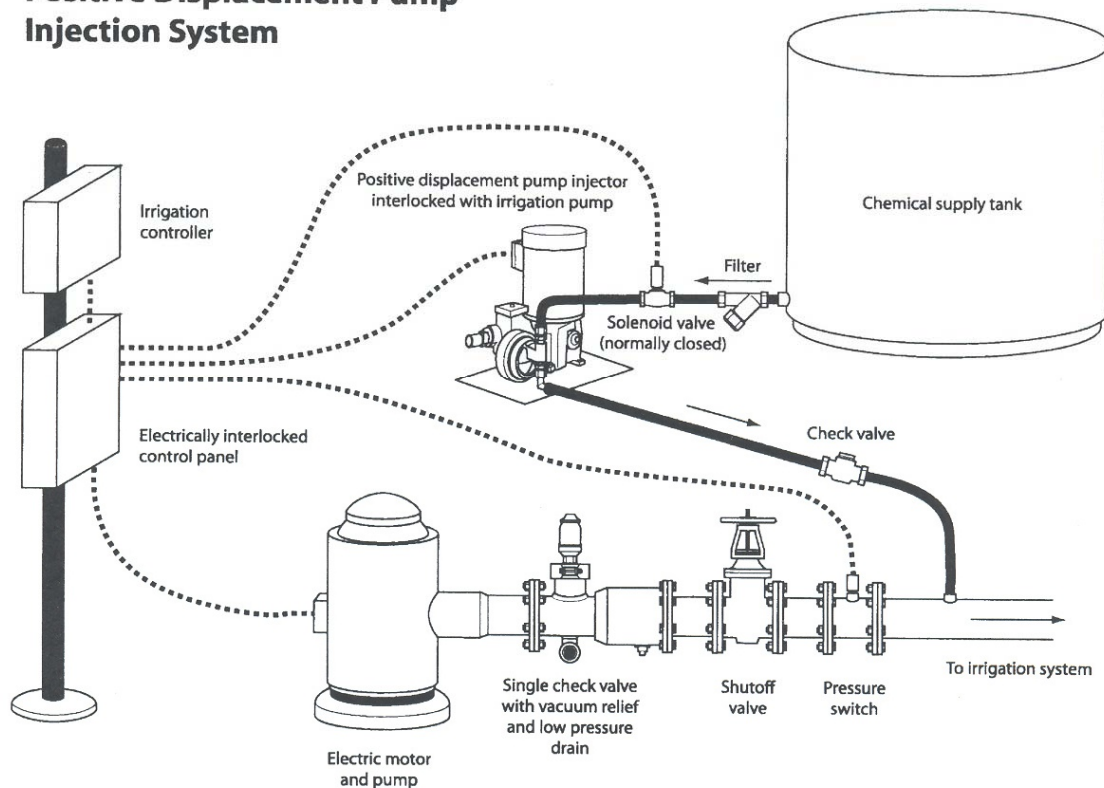
Figure 5. Layout of an Injection System with Safety Interlocks and Backflow Prevention Devices (Courtesy of L.J. Schwankl, Univ. of California-Davis)
