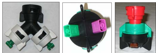
Figure 4. Double nozzle body adapter TeeJet Duo (left), Greenleaf TwinFan AirMix (center), and Greenleaf TurboDrop Venturi TwinFan (right). Twin fan uses the Hypro Twin-cap.
