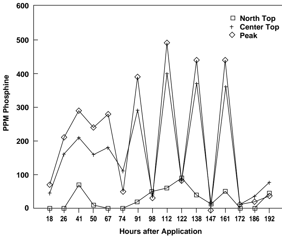
Figure 30. Phosphine gas concentrations at the top sampling points in a 10,000-bushel lot of grain sorghum when fumigant was applied at ground level.
