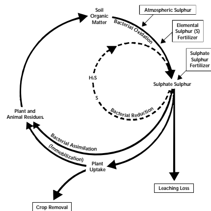
Figure 1. The Soil Sulphur Cycle
