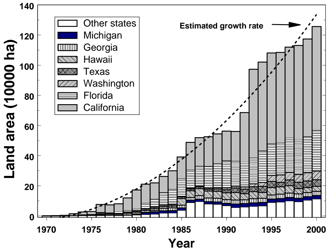
Figure 1.3. Microirrigation land area and distribution in the United States from 1970 through 2000. Based on surveys conducted by Irrigation Journal.
