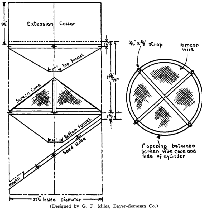
FIG. 16.—Oil barrel gravity seed treater, to be used in applying New Improved Ceresan only.
