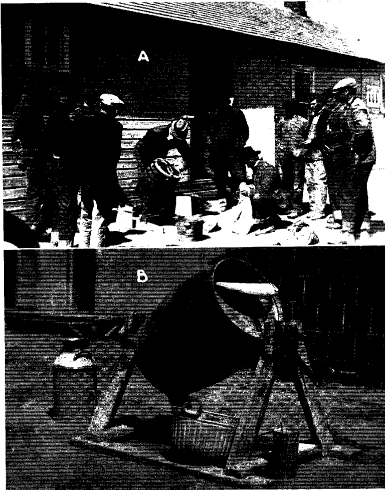
FIG. 12.—Dust treating outfits for smut control. (A) Churn used to treat small seed lots. (B) Homemade barrel treater.
