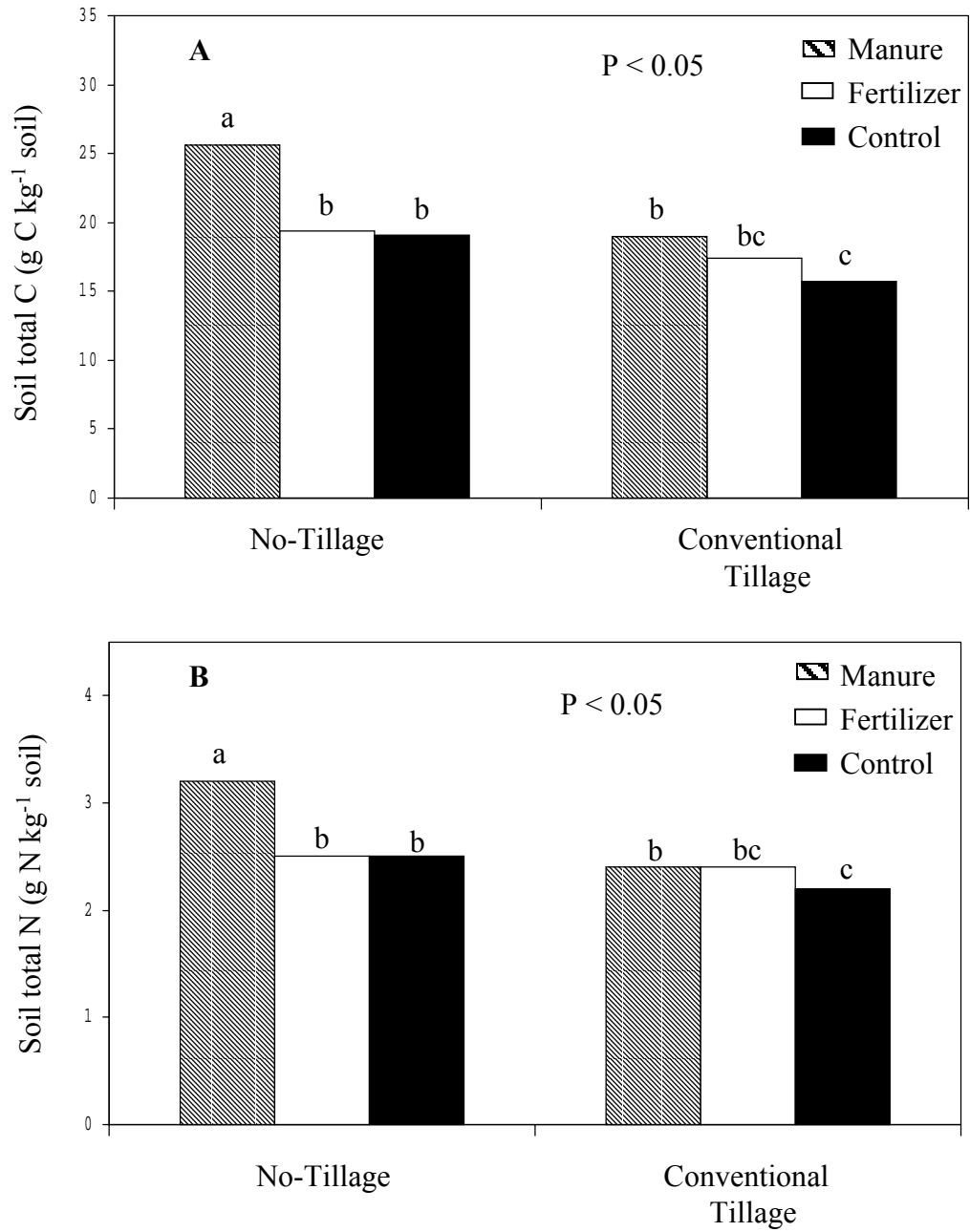
Figure 1: Soil total C and N. A represents soil total C; and B represents soil total N
