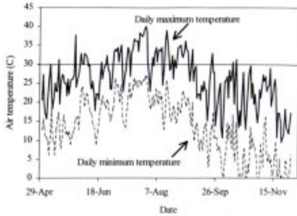
Fig. 1. Seasonal changes of daily maximum and minimum air temperatures.
