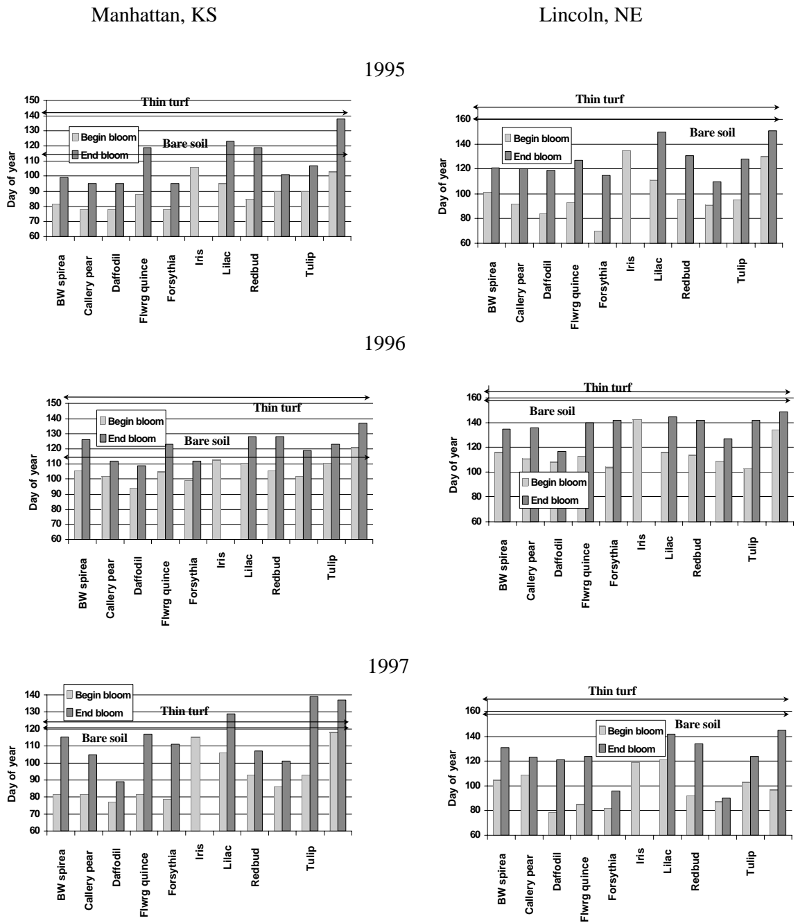
Figure 1. Correlation between a date 2 weeks prior to crabgrass emergence and the start and end of bloom of tested ornamental perennials.
