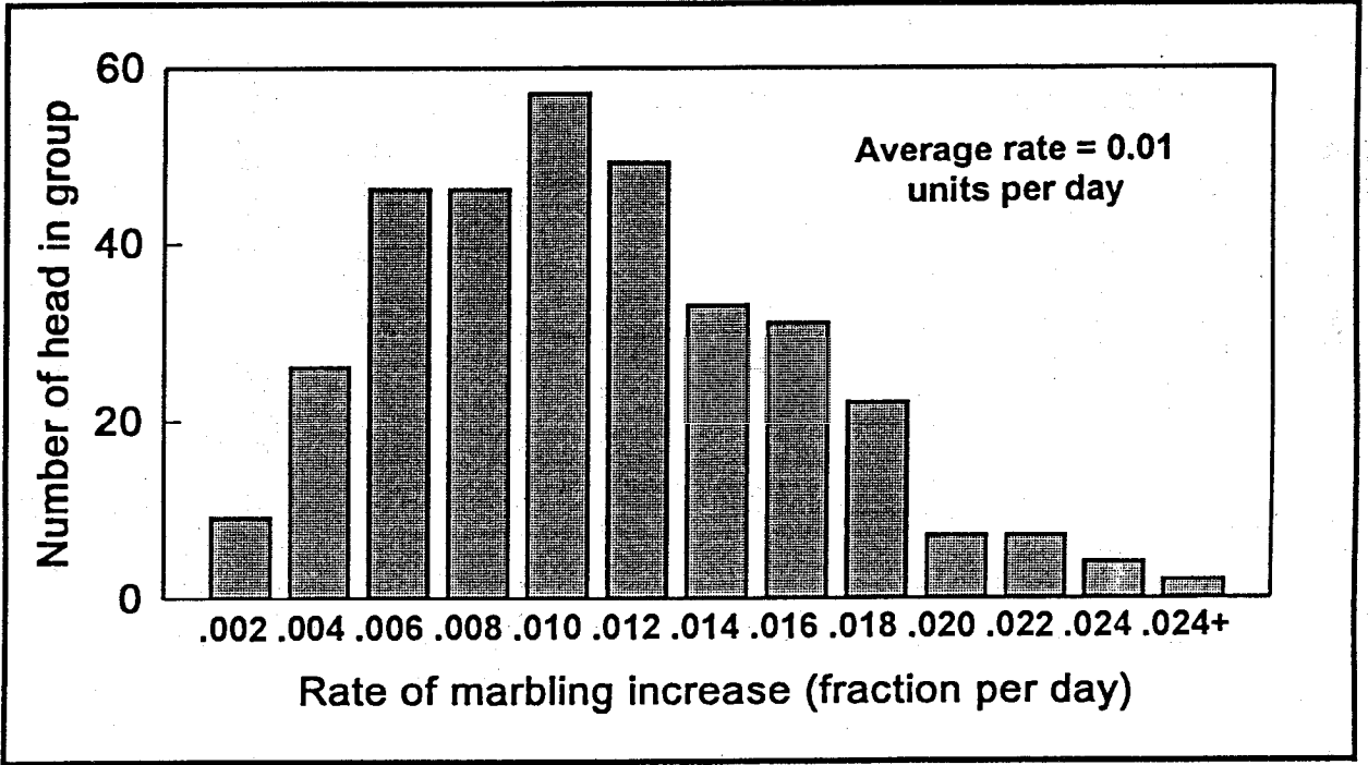
Figure 4. Distribution of marbling rates among 338 steers.
