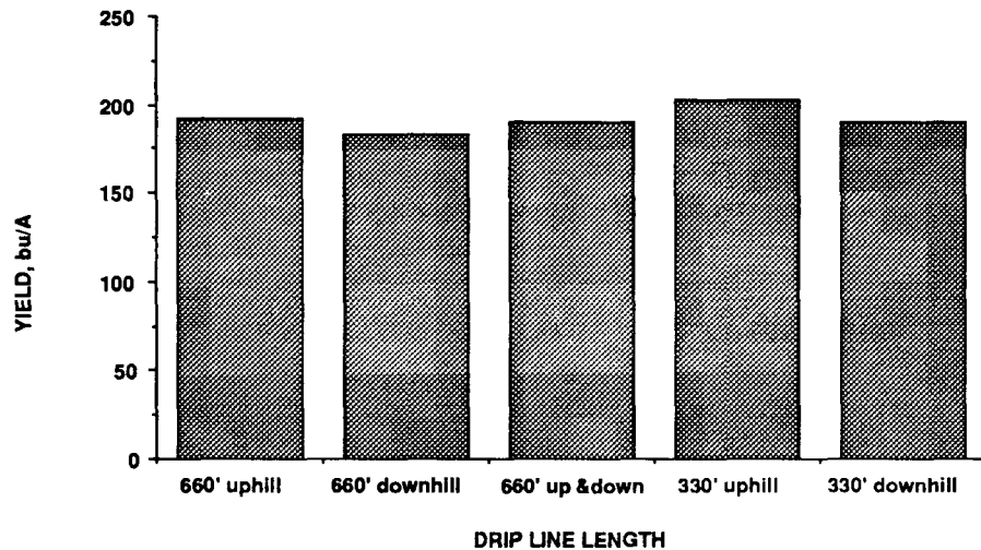
Figure 1. Drip irrigated corn yields as affected by line length and direction of water flow.
