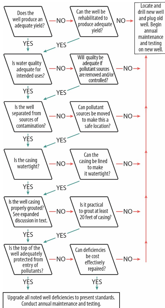
Figure 4. Well upgrade or replacement decision diagram
