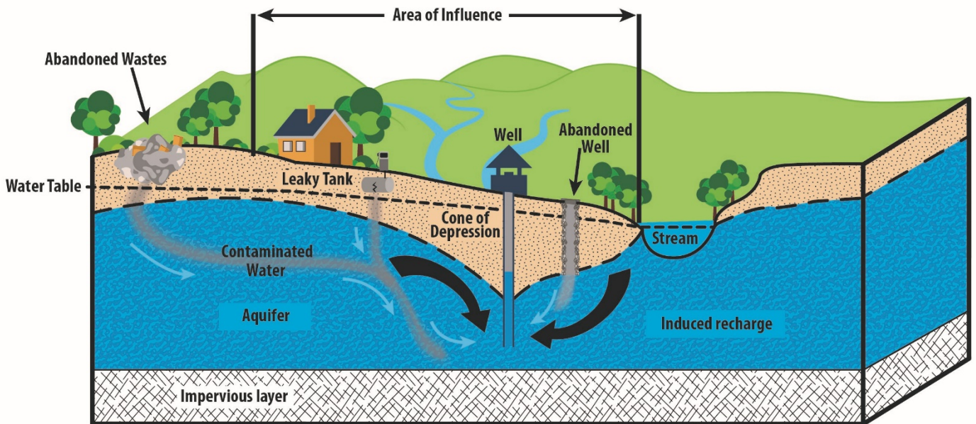
Figure 1. Cone of depression for a pumping well
